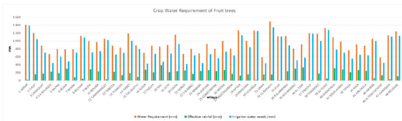
Fig. (4a). Crop water requirement (mm) of Fruit crops in Algeria.
